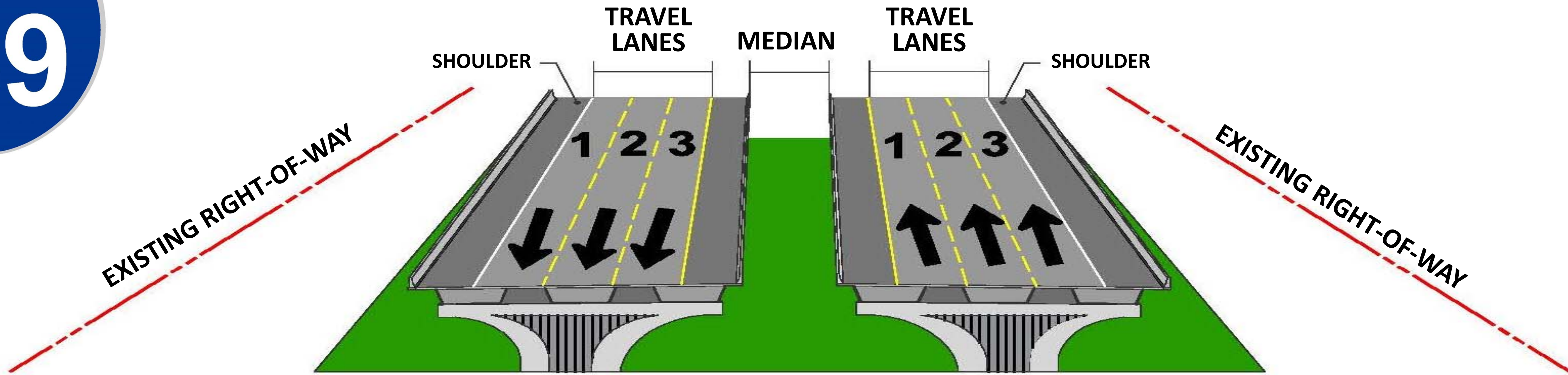
BUILD ALTERNATIVES 1 THROUGH 4 PROPOSED CONCEPT CROSS-SECTION
