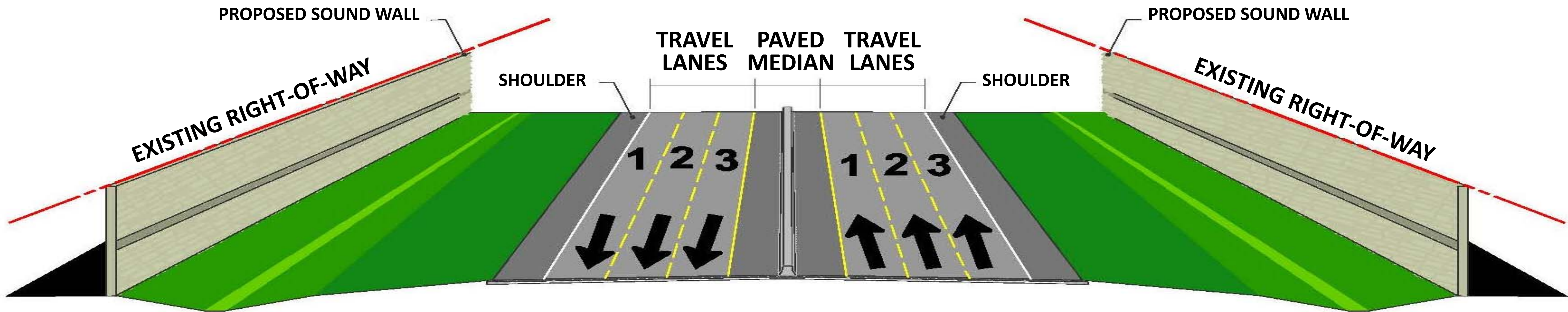
BUILD ALTERNATIVES 1 THROUGH 4 PROPOSED CONCEPT CROSS-SECTION
