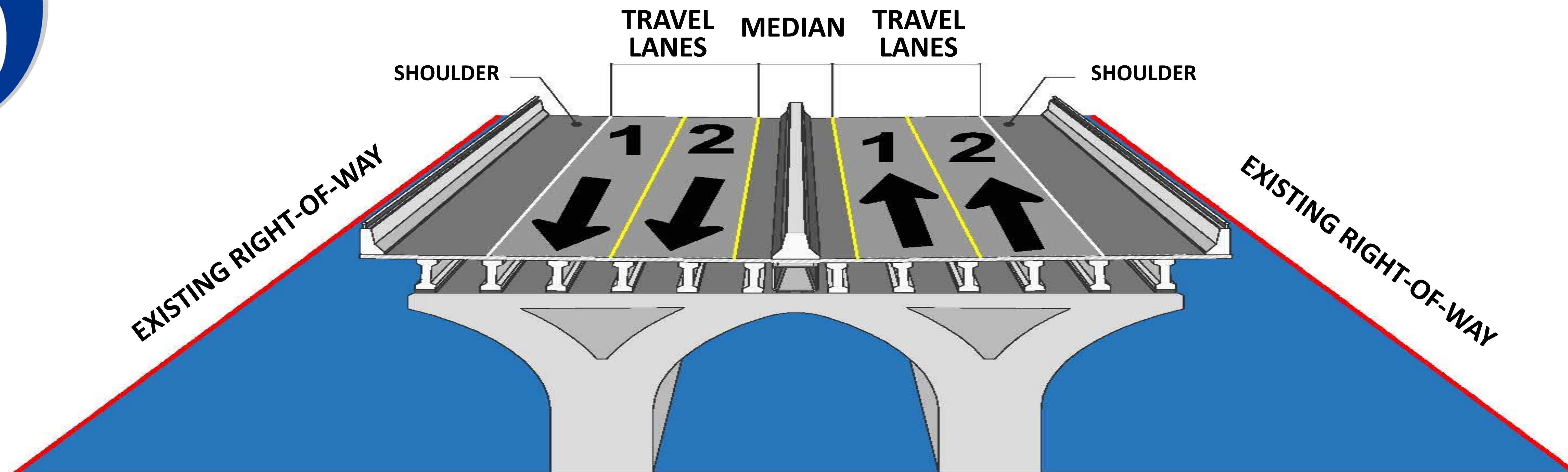
CROSS LAKE BRIDGE EXISTING CONDITIONS CROSS-SECTION
