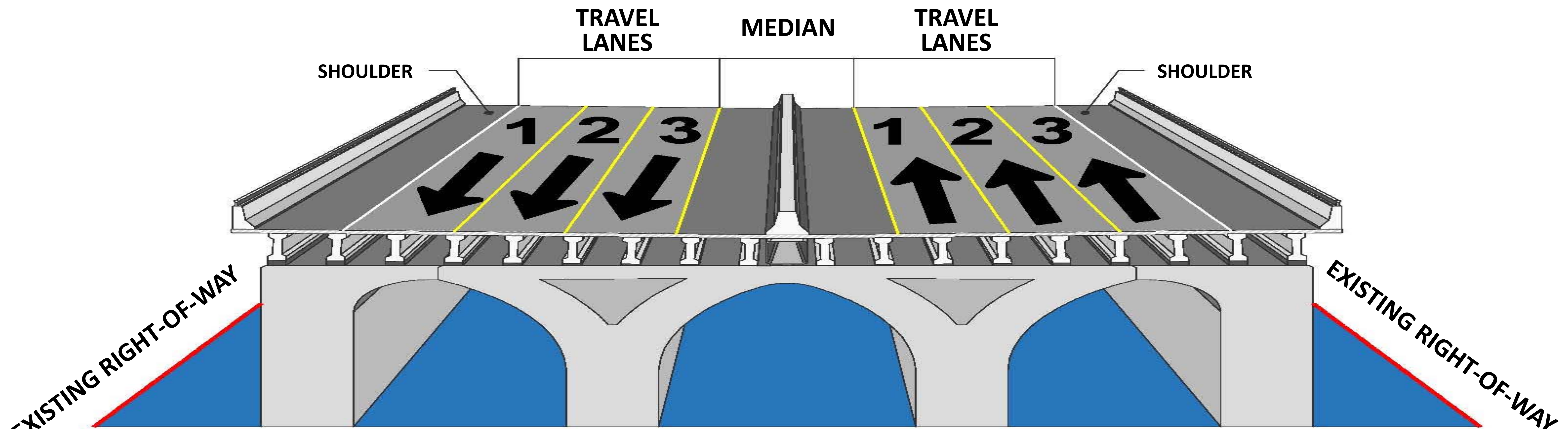
BUILD ALTERNATIVE 5 PROPOSED CONCEPT CROSS-SECTION
