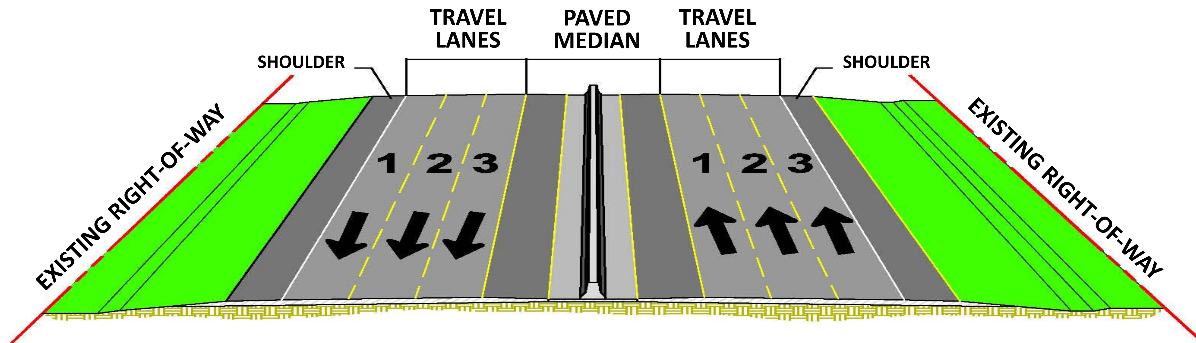
BUILD ALTERNATIVE 5 PROPOSED CONCEPT CROSS-SECTION
