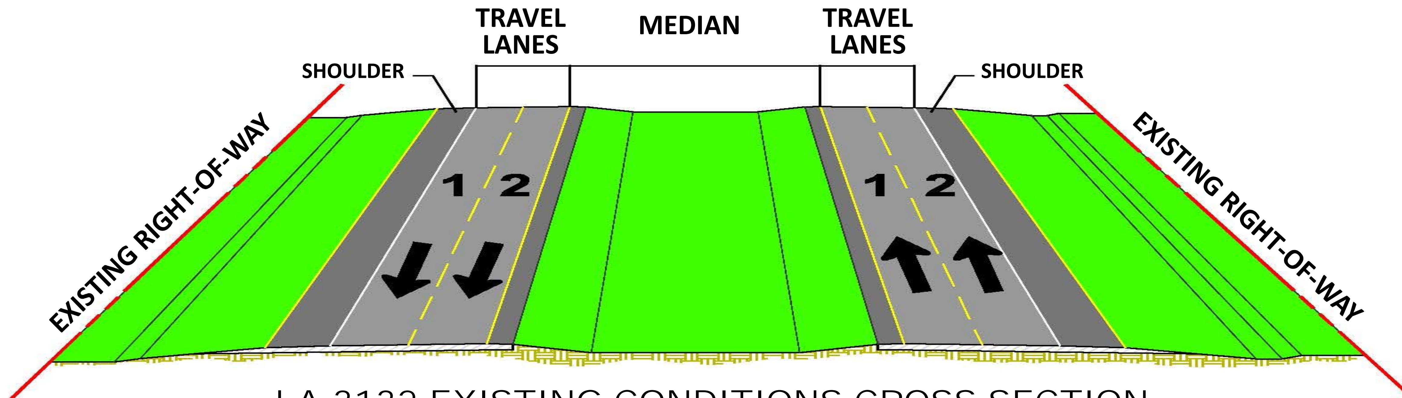
LA 3132 EXISTING CONDITIONS CROSS-SECTION
